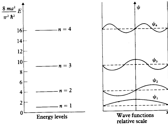
2.2 (a) The infinite square well (b) Wave functions and eigenvalues for the infinite square well.
